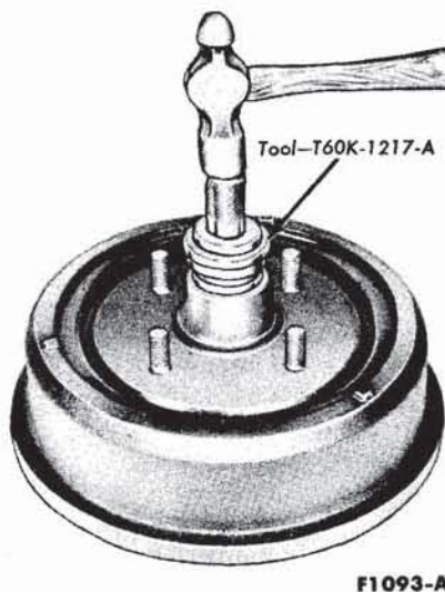
FIG. 5—Front Wheel Bearing Cup Installation
