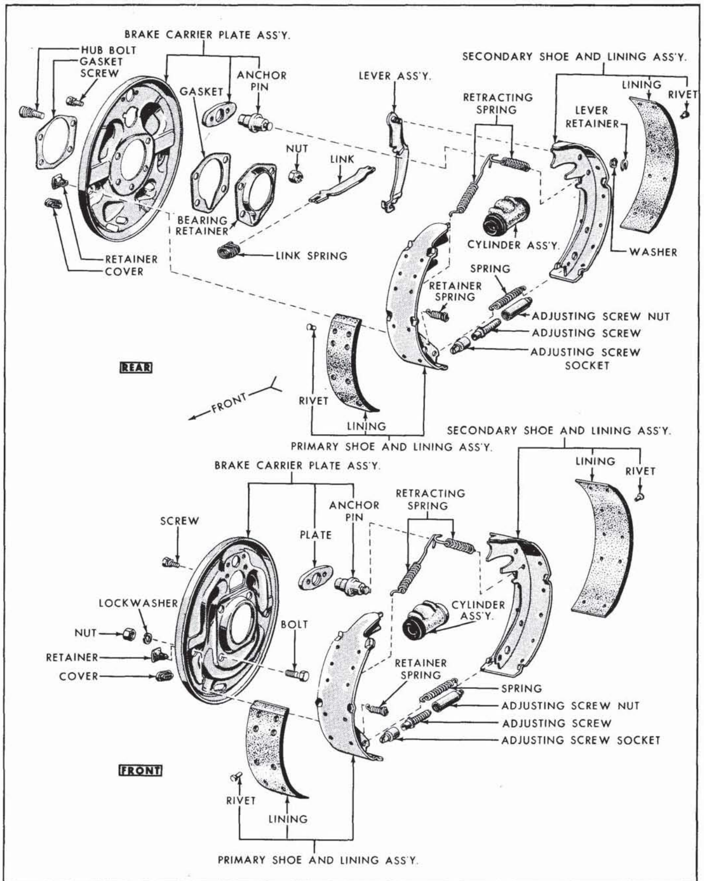
FIG. 1—Front and Rear Brakes—Disassembled—(60C-2009)
